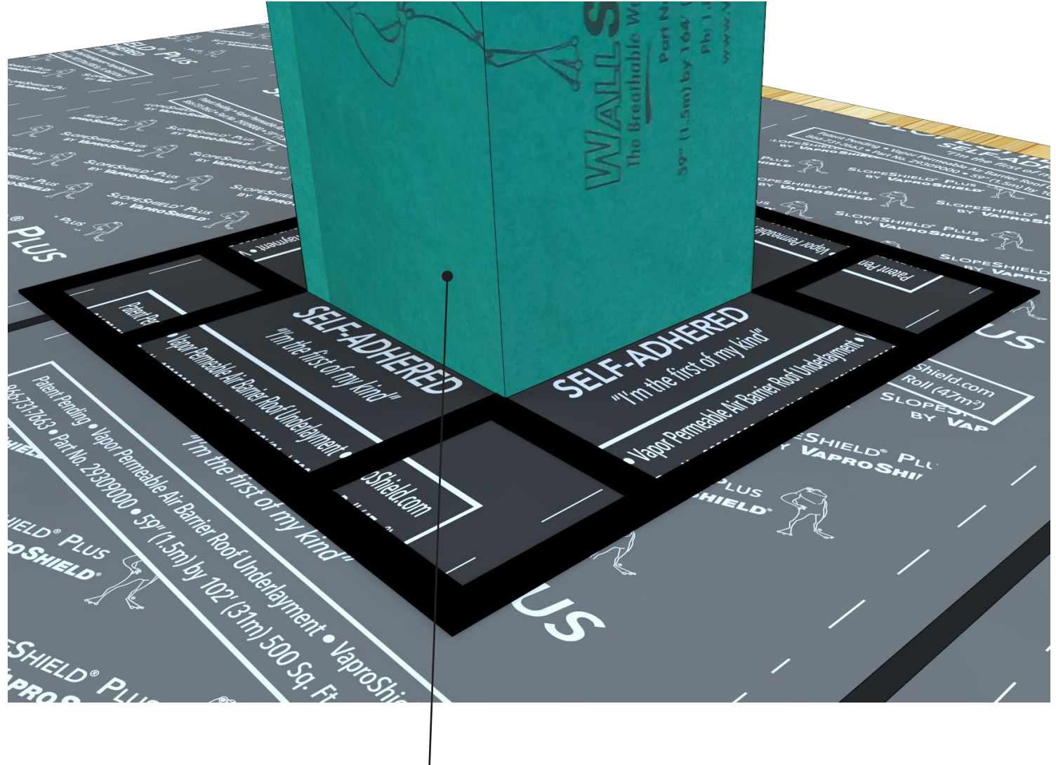
Install WallShield IT over post protection to optimize mass timber protection
