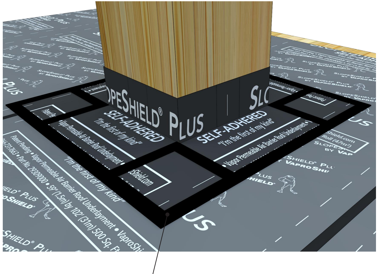
Apply VaproTape over all seams and edges of SlopeShield Plus SA.
